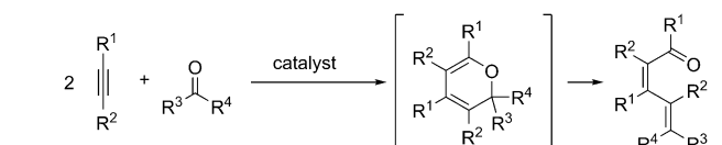
Scheme 1. Transition-metal-catalyzed [2+2+2] cycloaddition reactions of alkynes and carbonyl compounds.
