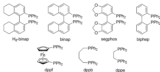
Scheme 2. Structures of bisphosphine ligands.
