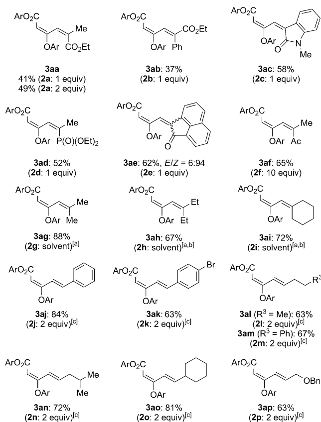
Scheme 3. Rhodium-catalyzed [2+2+2] cross-trimerization reactions of ethynyl 2-naphthyl ether ( 1a ) and carbonyl compounds 2a–p . [Rh(cod) 2 ] 2 BF 4 (0.0075 mmol), H 8 -binap (0.0075 mmol), 1a (0.30 mmol), 2a–p (0.30–3.0 mmol), and CH 2 Cl 2 (2.0 mL) were used. Cited yields are of the isolated products. [a] 2g–i were used as a solvent instead of CH 2 Cl 2 . [b] [Rh(cod) 2 ] 2 BF 4 (0.015 mmol) and H 8 -binap (0.015 mmol) were used. [c] (CH 2 Cl) 2 was used as the solvent.
